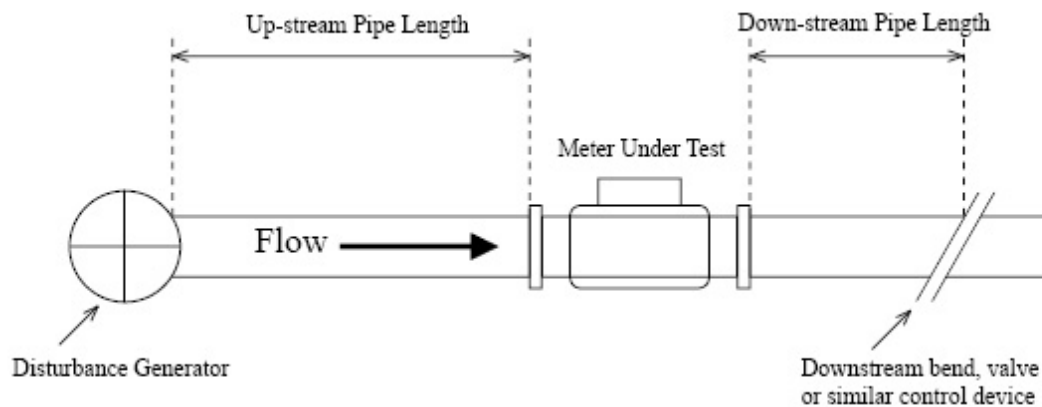
Figure B.4. Test set-up
