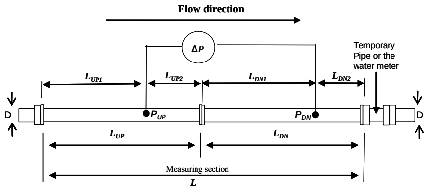
Fig 1: Pressure loss test; Layout of measuring section
