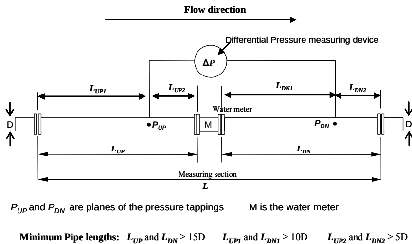
Fig 1: Pressure loss test; Layout of measuring section
