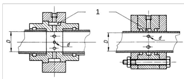
Figure D.1. Example of drilled hole type of pressure tapping with ring chamber, suitable for small/medium diameter test sections (1 is the ring chamber)
