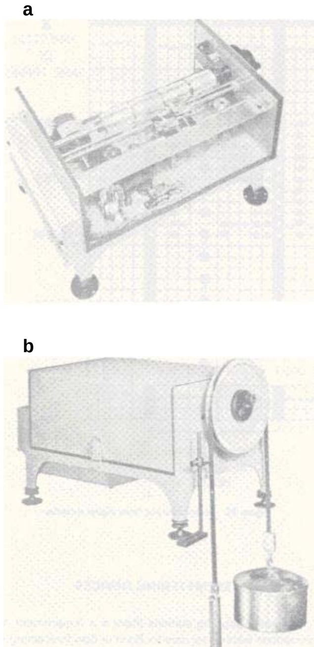
Figure 33. a) Stevens Telemark with coding bar and switch for signalling radio station identification call letters and numerals in International Morse Code and b) float-operated Telemark (Courtesy of Leupold & Stevens Inc.).
