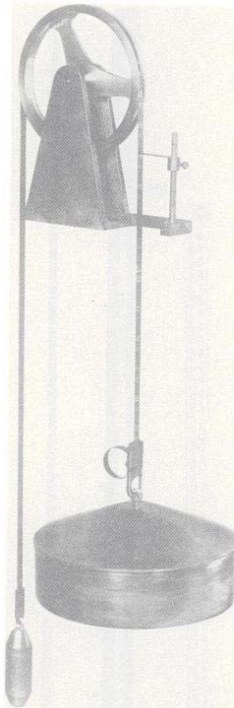
Figure 6. Float gauge (Courtesy of Leupold & Stevens Inc.).
