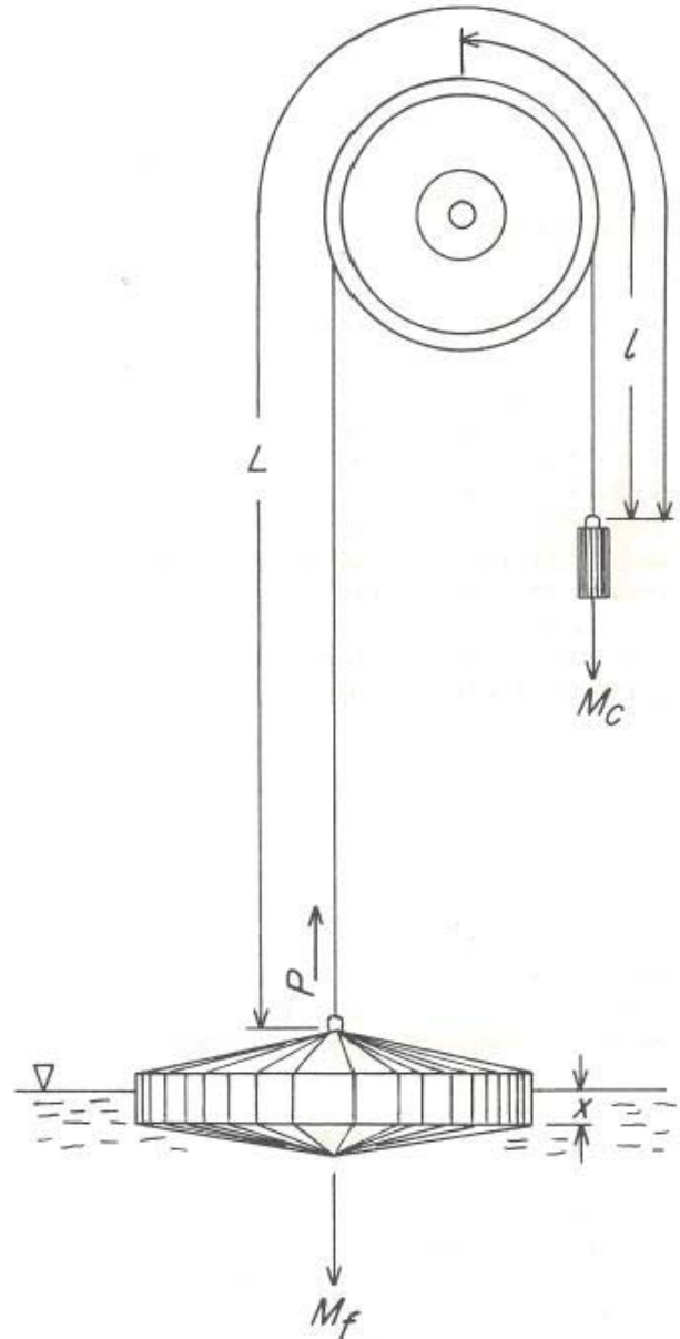
Figure A- 1. Typical float system.
