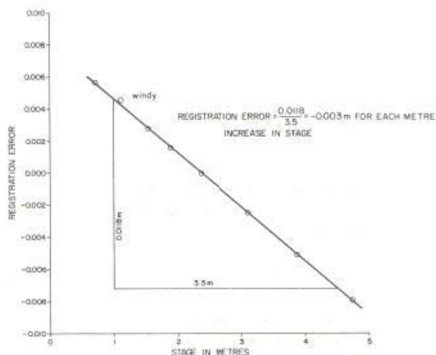
Figure 28. Servomanometer correction.
