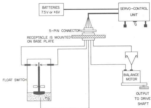
Figure 26. Servomanometer.
