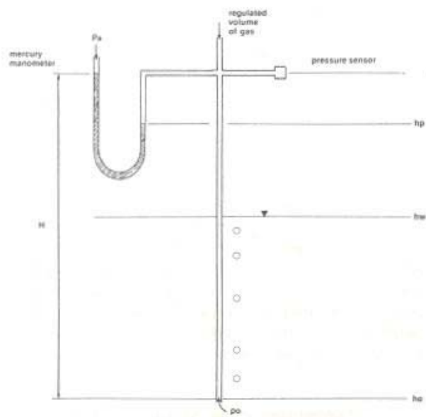
Figure B- 1. Gas purge system with stage sensors.
