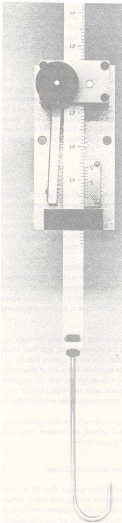
Figure 4. Hook gauge (Courtesy of Leupold & Stevens Inc.).
