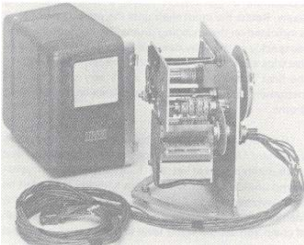
Figure 34. Memomark 11.
