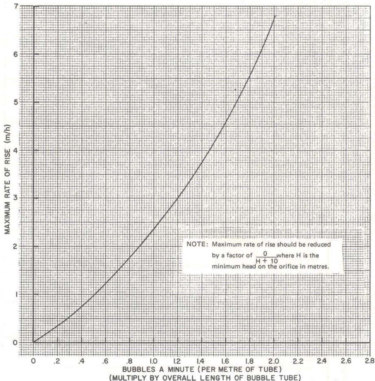
Figure 20. Graph for calculating bubble feed rate.
