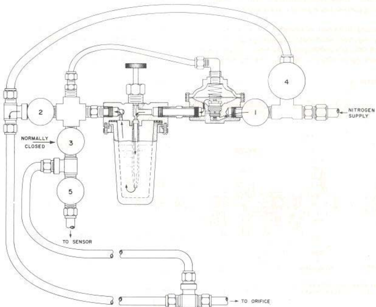
Figure 16. Gas purge system (dual line).
