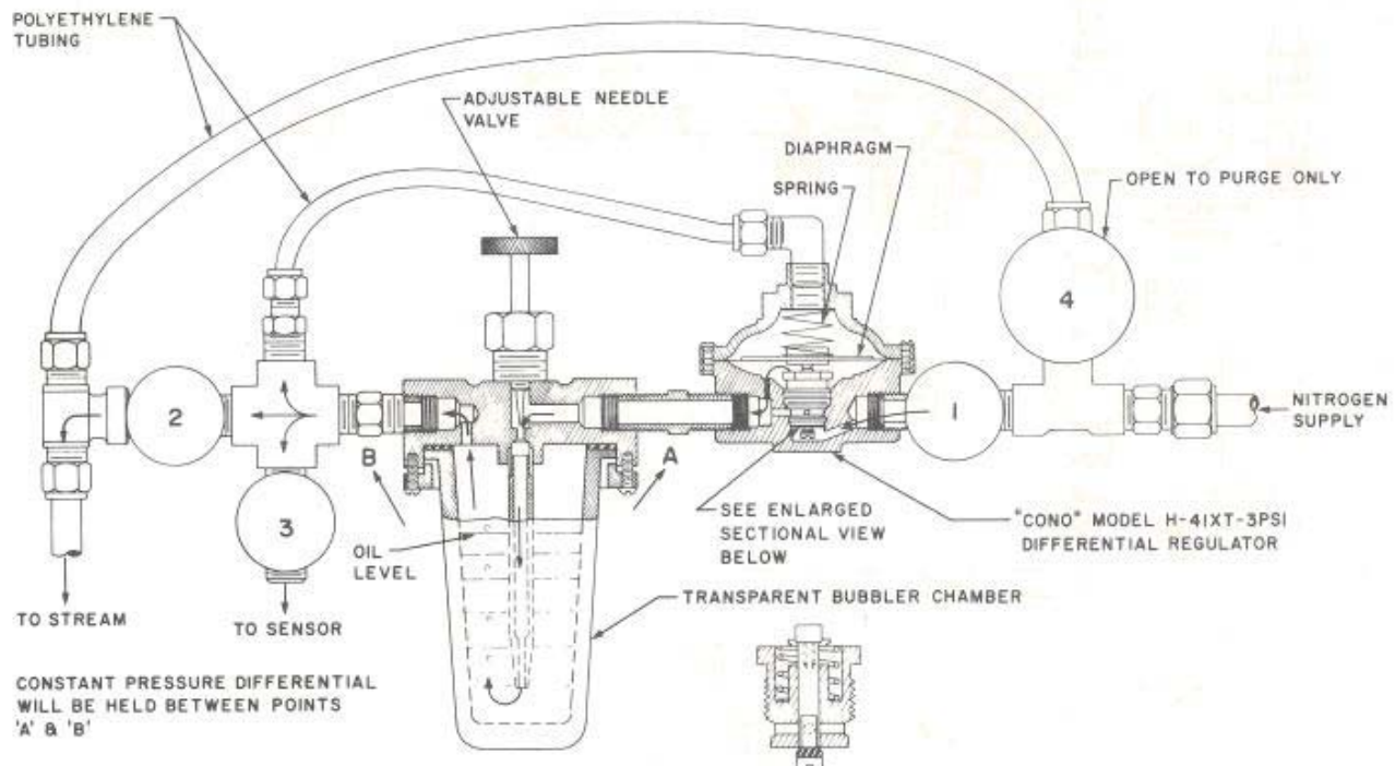
Figure 13. Details of Conoflow differential pressure regulator
