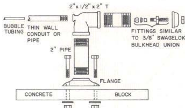
Figure 18. Conventional orifice assembly.
