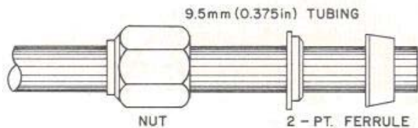
Figure 19. Assembly of Swagelok fittings.
