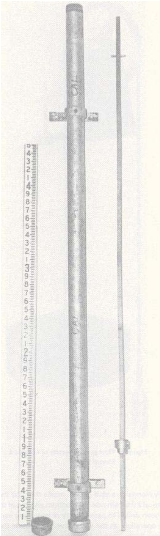
Figure 7. Crest stage gauge (USGS type).
