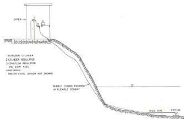
Figure 14. Typical gas purge system installation.
