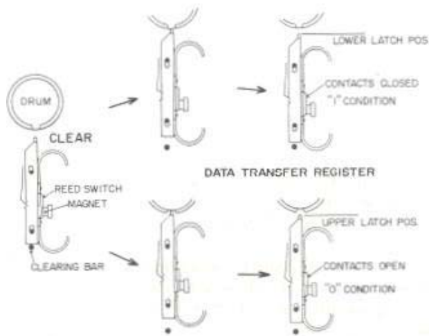
Figure 36. Memomark encoding cycle.
