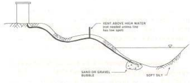
Figure 15. Well point orifice.
