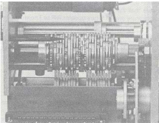
Figure 35. Memomark encoding assembly.
