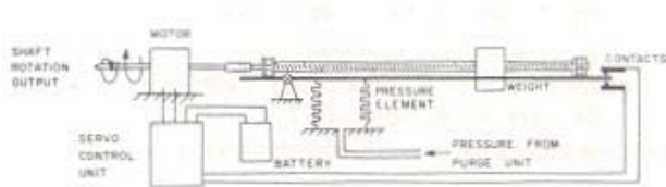
Figure 30. Servo-beam-balance principle.
