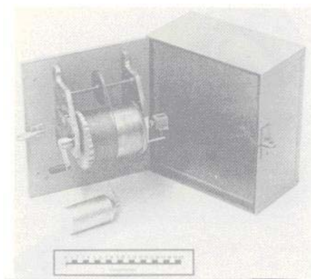
Figure 3. Wire weight gauge (counter type).
